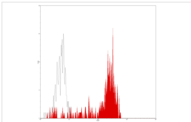
Human peripheral blood monocytes analyzed with Purified CD14 mAb, followed by anti-mouse IgGs-PE
