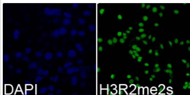
Immunofluorescence analysis of 293T cell using H3R2me2s antibody. Blue: DAPI for nuclear staining.
