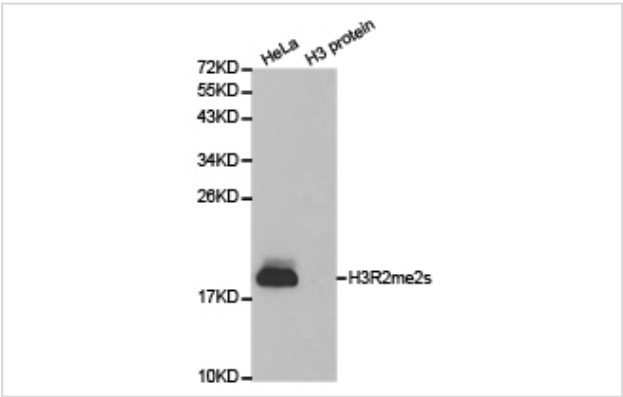
Western blot analysis of extracts of HeLa cell line and H3 protein expressed in E.coli., using H3R2me2s antibody.
