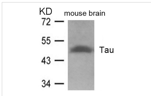
Western blot analysis of extracts from mouse brain tissue using Tau(Ab-262) Antibody #AB21100.
