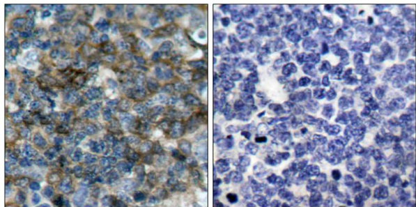
Immunohistochemical analysis of paraffin-embedded human tonsil carcinoma tissue using VASP(Phospho-Ser157) Antibody #AB11214(left) or the same antibody preincubated with blocking peptide(right).
