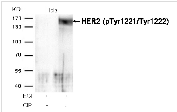
Western blot analysis of extracts from Hela cells, treated with EGF or calf intestinal phosphatase (CIP), using HER2 (Phospho-Tyr1221/Tyr1222) Antibody #AB11076.
